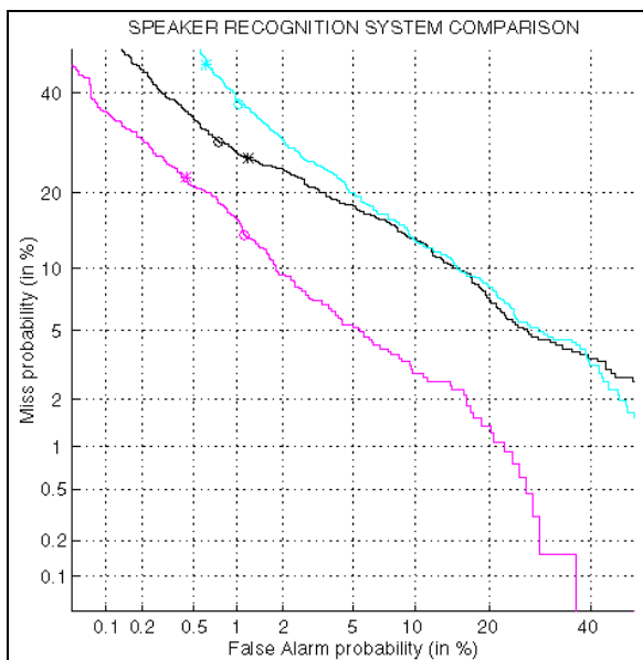
Figure 1: Plot of DET Curves for a speaker recognition evaluation.
